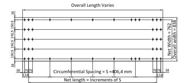
Fig. 1. Geometry of SuperCor® plate (total length, i.e. multiple S=406,4 mm)
