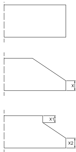
Fig. 6. End finishes of SuperCor®
