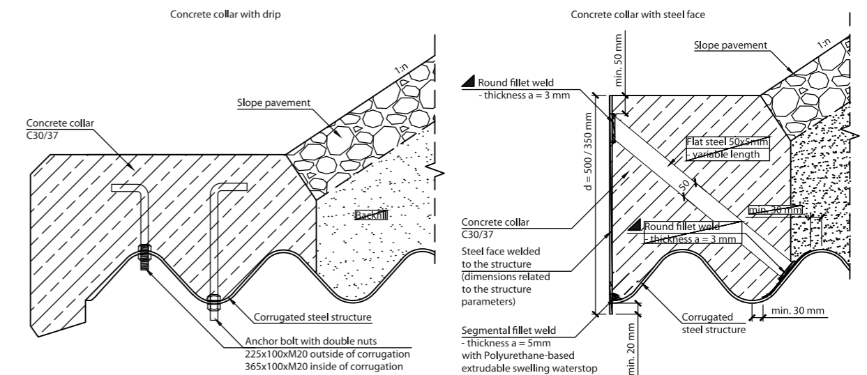
Fig. 12. Example of a concrete collar on inlet and outlet of the structure
