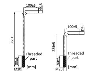
Fig. 3 Anchor bolts used to mount structure in foundation
