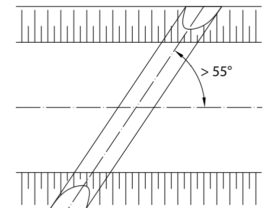
Fig. 2. Skewed structure
