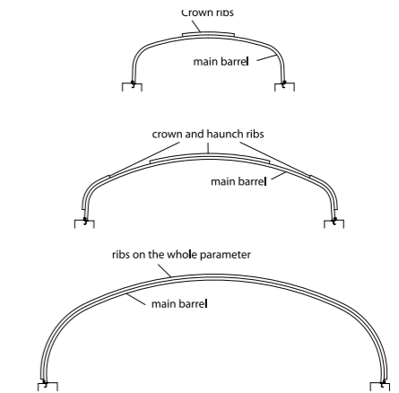
Fig. 8. Placement of the ribs in cross section of the structure
