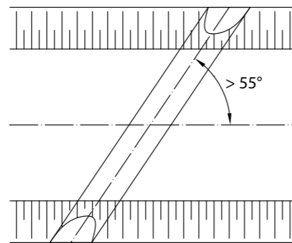
Fig. 7. Skewed structure
