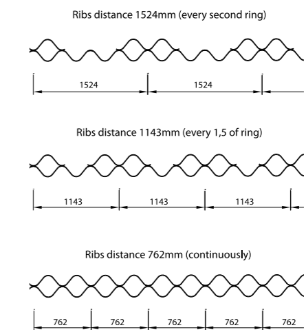
Fig. 9. Placement of the ribs in longitudinal direction of the structure
