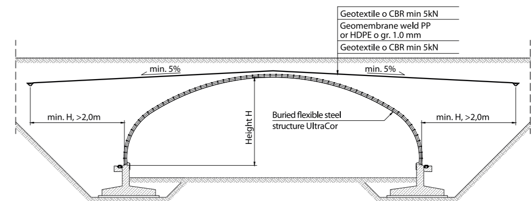
Fig 10. Scheme of rainwater protection
