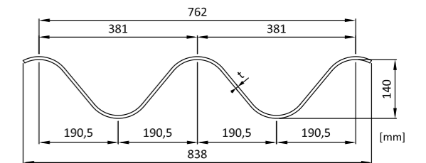
Fig. 2. Cross section of SuperCor® plate
