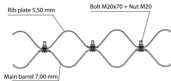
Fig. 5. Connection of ribs to main barrel plates
